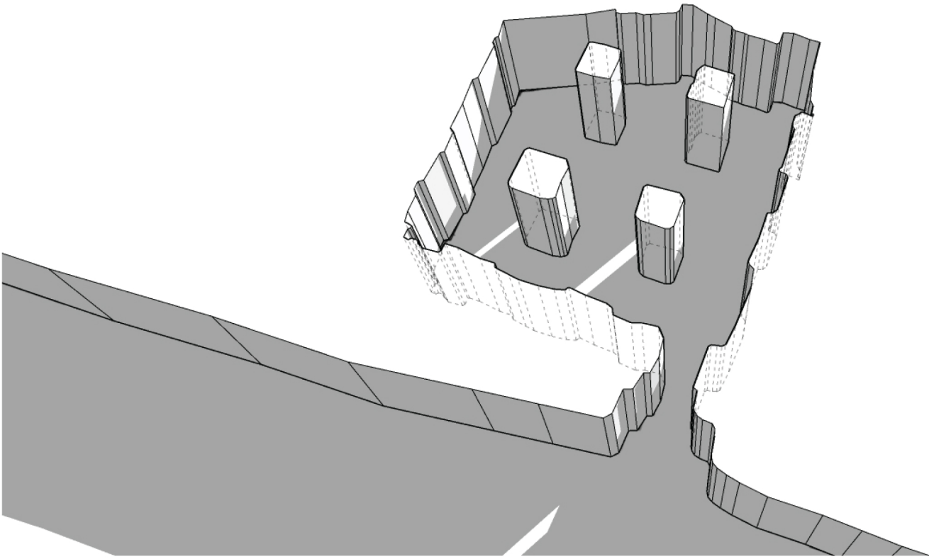
Axonometric layout of the excavation
